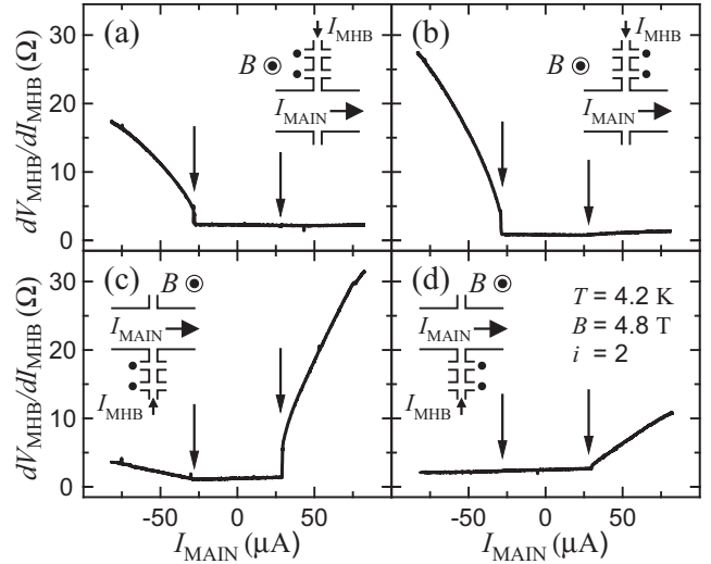
FIG. 3: Differential longitudinal resistance dV_{\text{MHB}}/dI_{\text{MHB}} with I_{\text{MHB}} = 0.2 \mu\text{A} in the upper ((a) and (b)) and lower ((c) and (d)) micro Hall bars as a function of electric current I_{\text{MAIN}} through the main channel. The critical current obtained from Fig. 2 is indicated by arrows. The black dots in the insets indicate the voltage probes used in the measurements.
